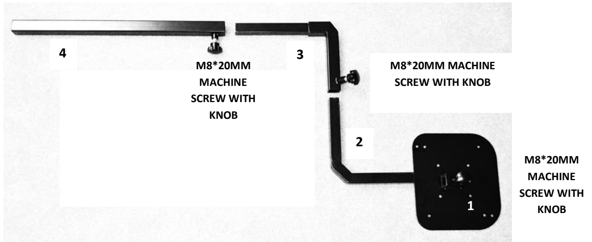
FIGURE 9C: CENTER MOUNT
